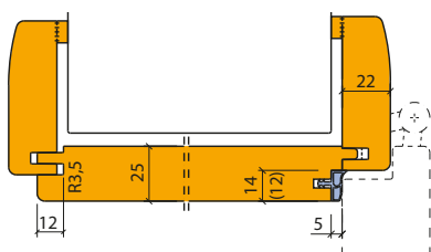
Door lining profile
