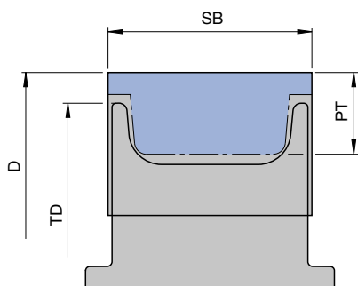
Tool body, U profile
