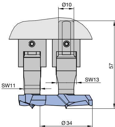
Double hinge drills in aggregate
